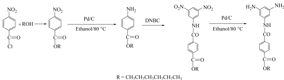
Scheme 1 The synthetic route to the functional diamine C6-PDA
