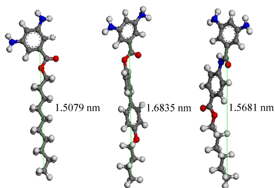
Fig. 2 Side chain lengths of diamines
