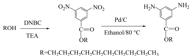
Scheme 2 The synthetic route to the functional diamine C10-DA
