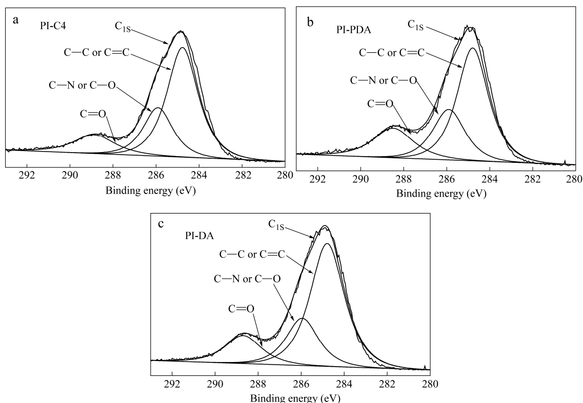
Fig. 7 XPS spectra of three kinds of PI (incident angle 10°)
