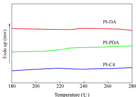
Fig. 4 DSC curves of PIs
