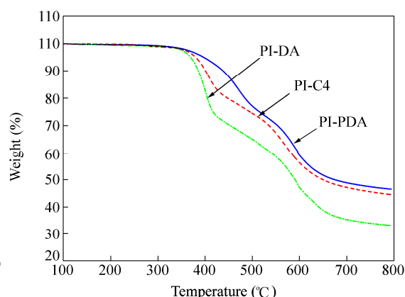
Fig. 5 TGA curves of PIs
