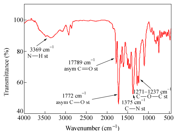
Fig. 1 FTIR spectrum of PI-PDA
