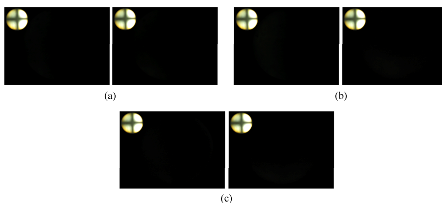
Fig. 6 POM images and conoscopic images before and after rotating by 45^\circ of LC cells: (a) PI-C4, (b) PI-PDA and (c) PI-DA
