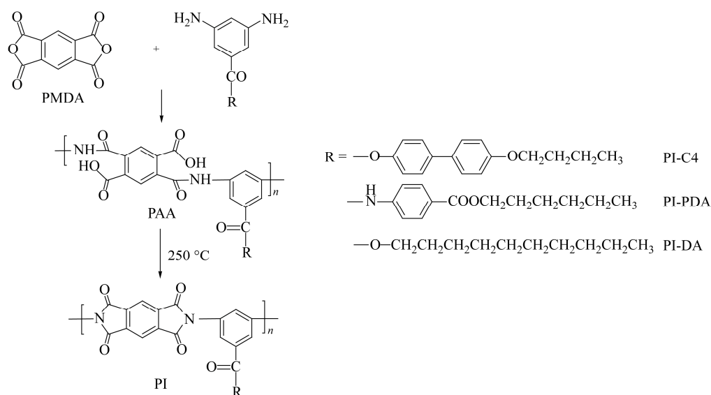
Scheme 3 The synthetic route to the three PIs
